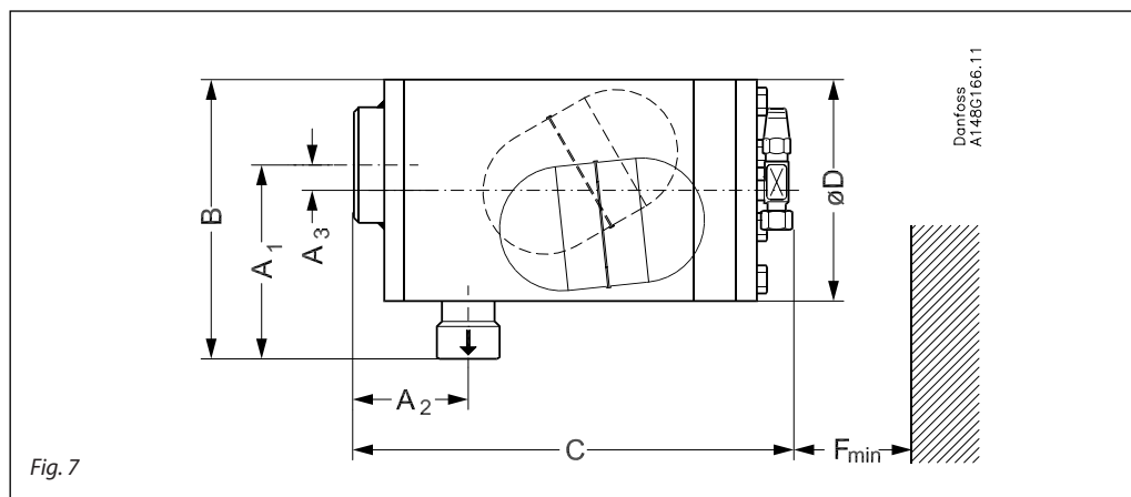
High pressure float valve without flange (Fig. 7)
