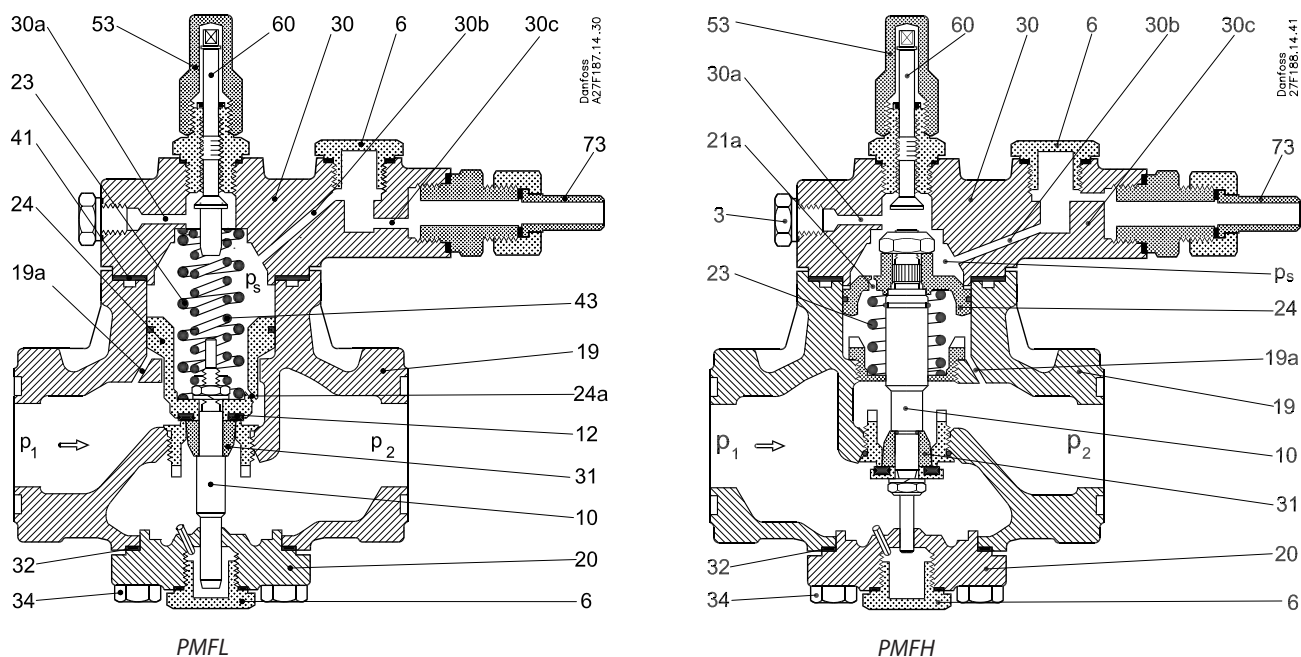
Material specification for PMFL/PMFH valves
