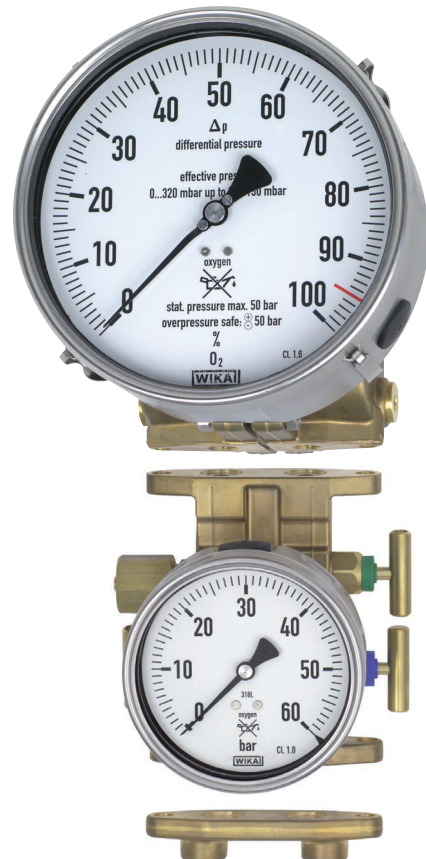
Fig. top: Differential pressure gauge model 712.15.160
