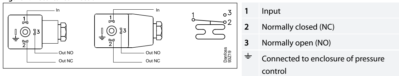
Figure 1: Electrical connection
