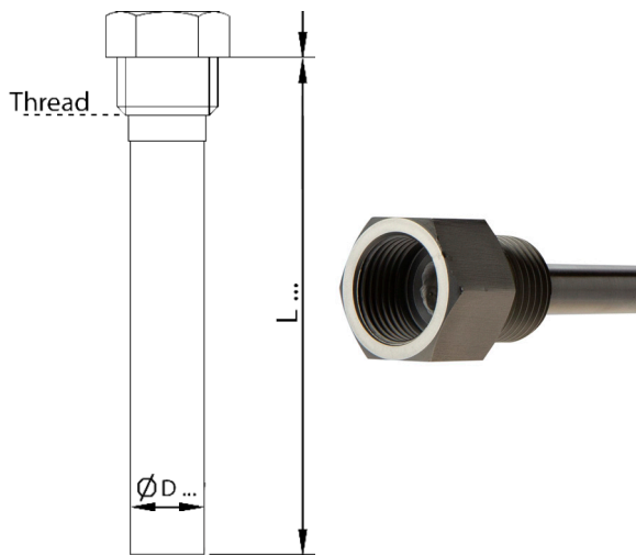
Model TW1 : Fixed thread connection
