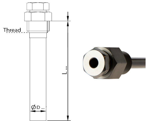
Model TW2: Sliding connection
